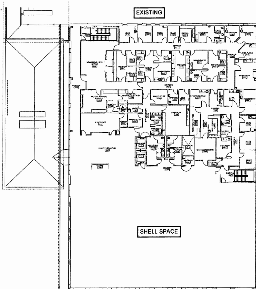
SECOND FLOOR PLAN - ACC CON Permit #14-056
