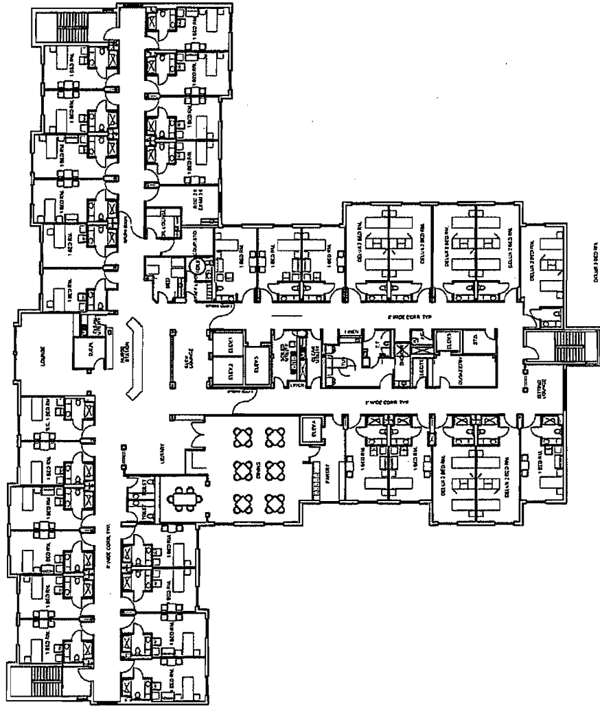
SECOND & THIRD FLOOR PLAN 22,300 sf (33 ROOMS, 40 BEDS) SCALE 3/32"=1'-0"
