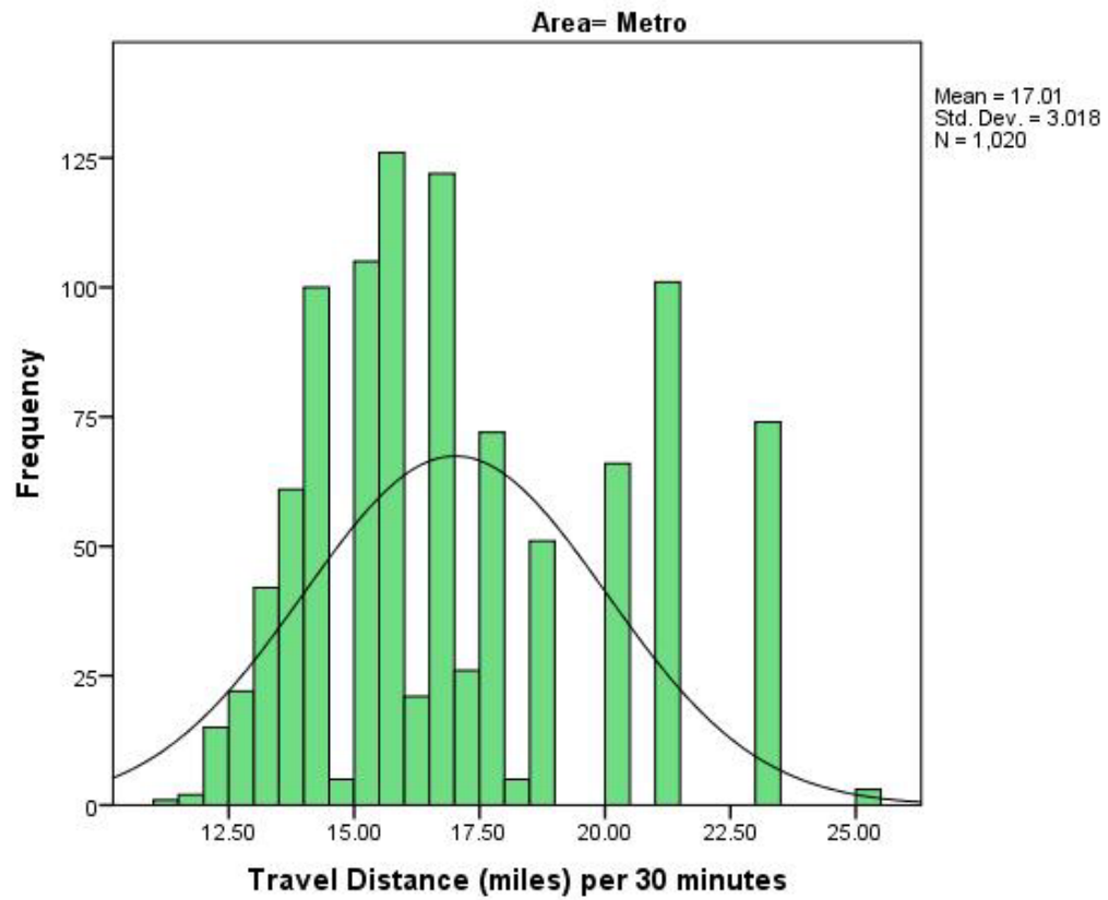
Figure 5: Distribution of sample travel distance means 30-minute drive in Metro area
