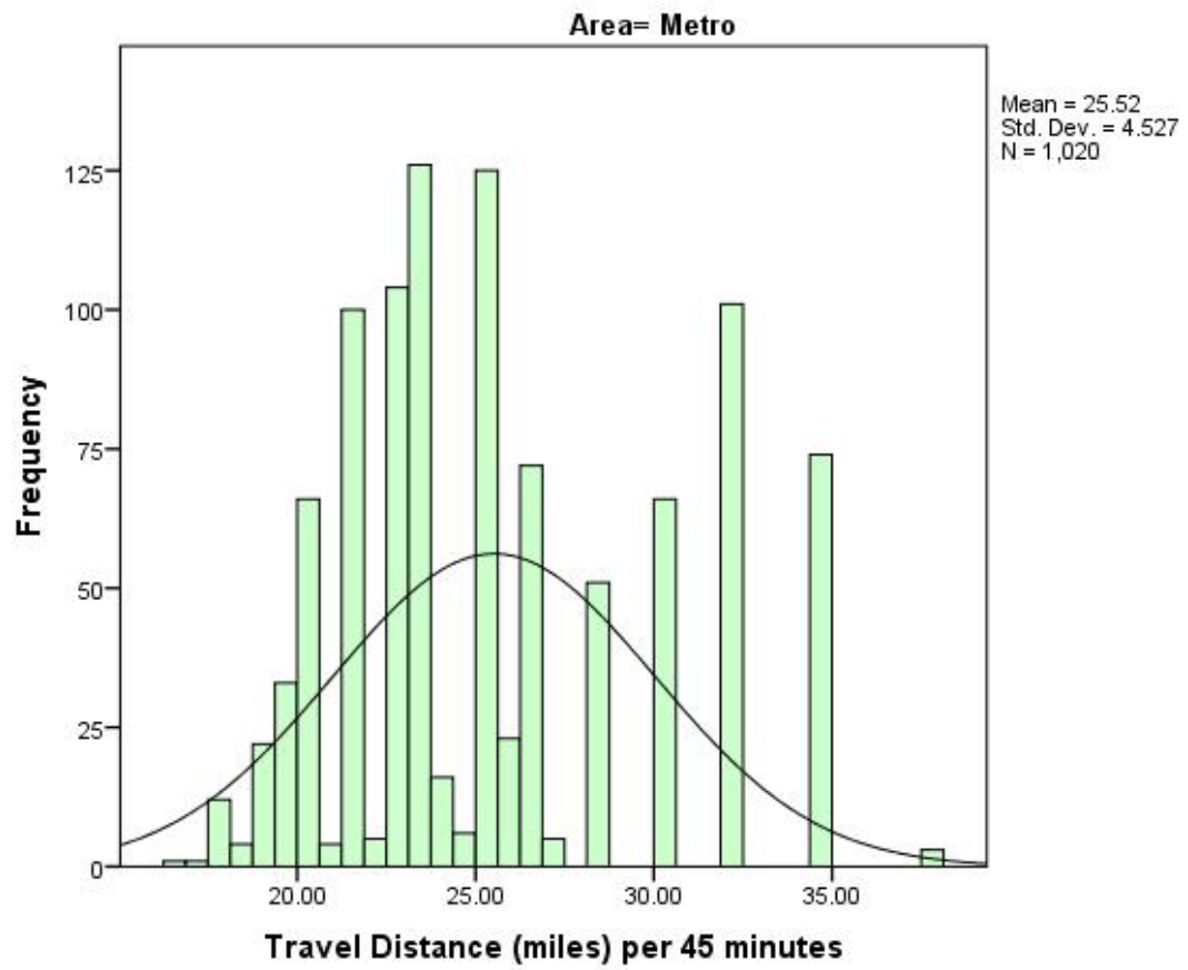
Figure 6: Distribution of sample travel distance means 45-minute drive in Metro area
