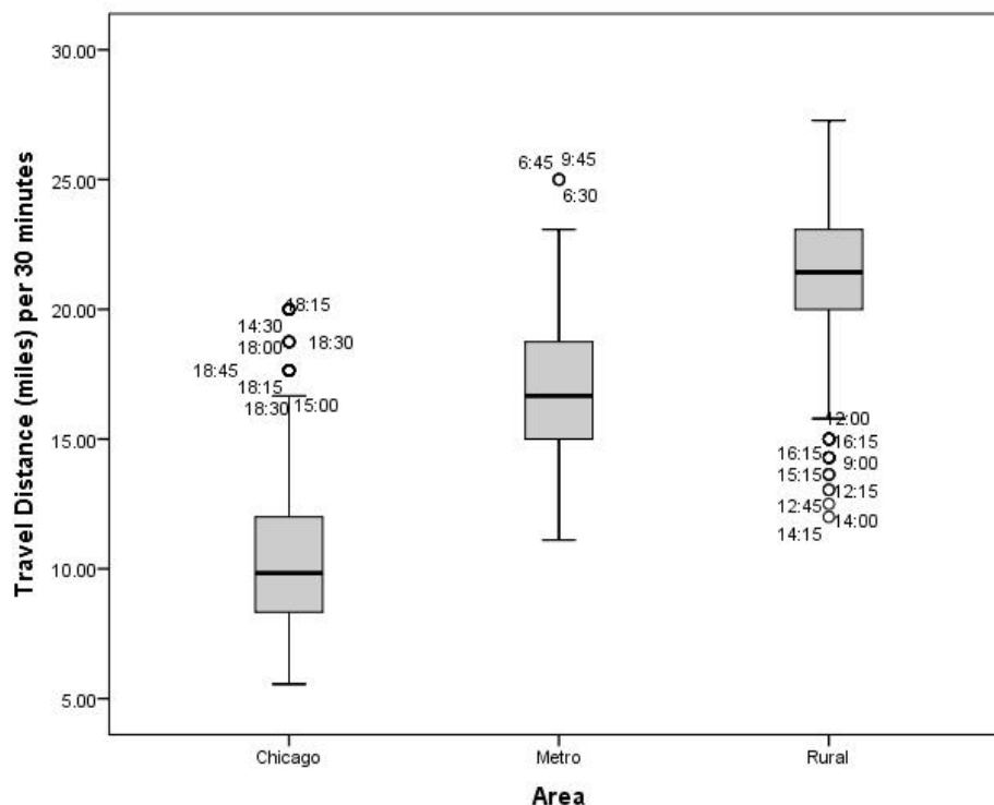
Figure 10: box plot showing travel distance outliers in Chicago, Metro, and Rural areas.
