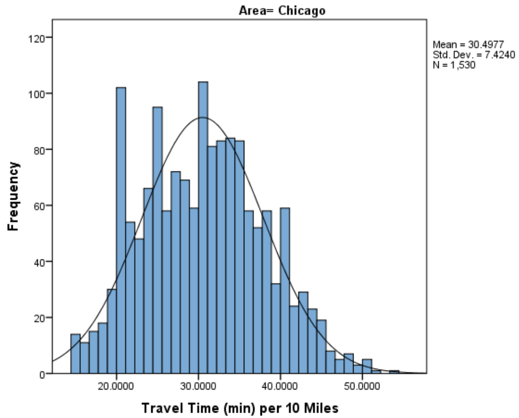
Figure 1: Distribution of sample travel time means for 10-mile drive in Chicago
