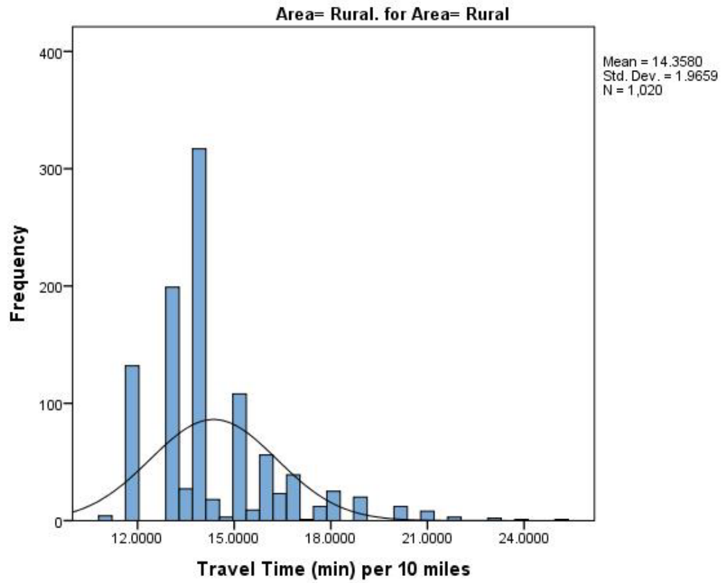
Figure 7: Distribution of sample travel time means for 10-mile drive in Rural area
