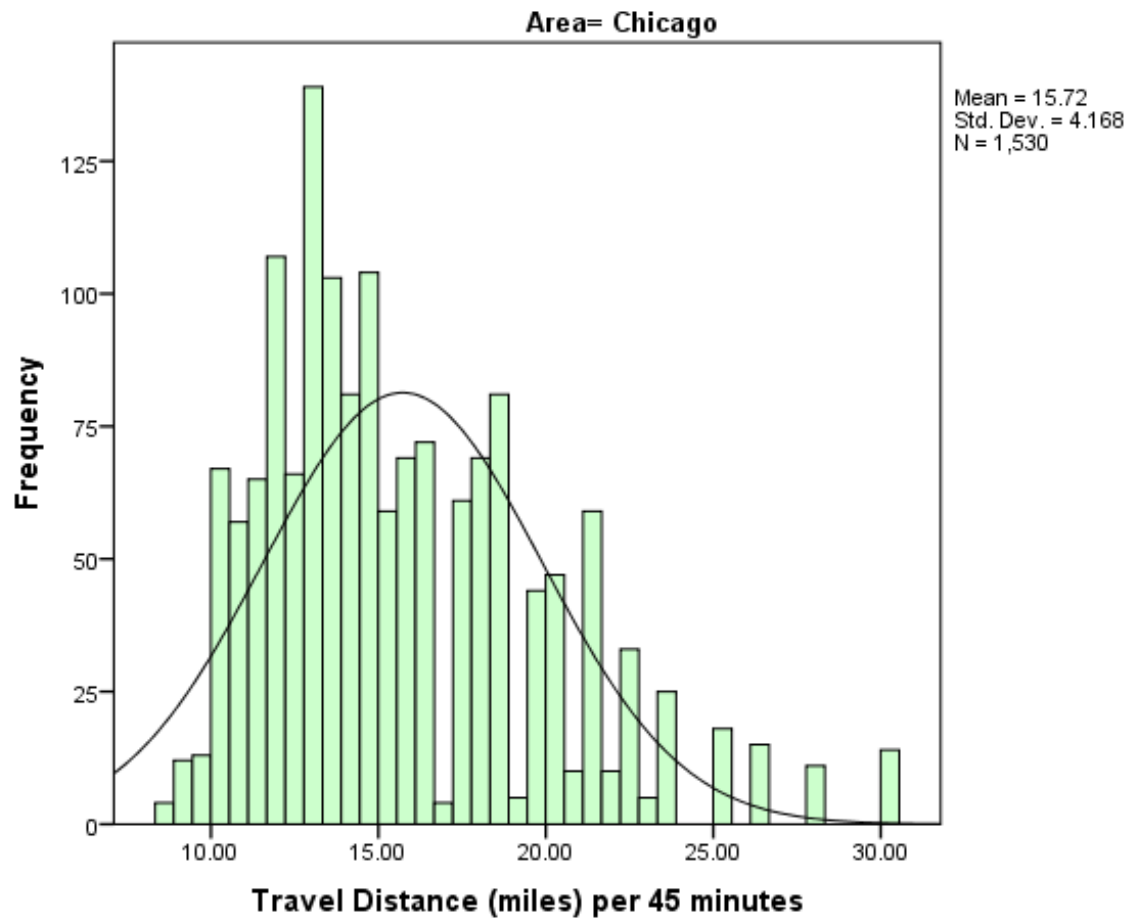
Figure 3: Distribution of sample travel distance means 45-minute drive in Chicago
