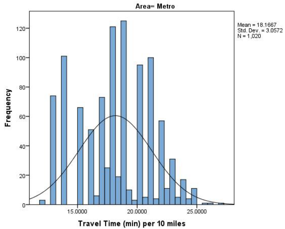
Figure 4: Distribution of sample travel time means for 10-mile drive in Metro area
