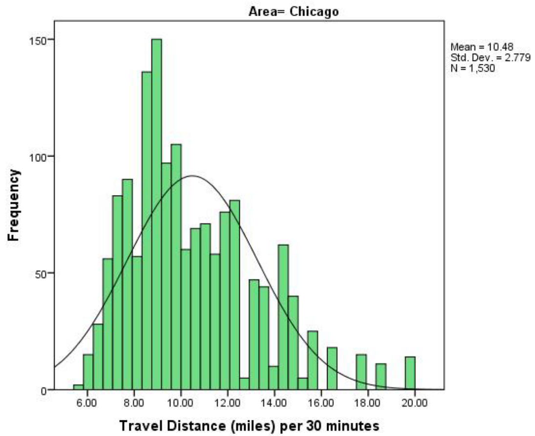
Figure 2: Distribution of sample travel distance means for 30-minute drive in Chicago
